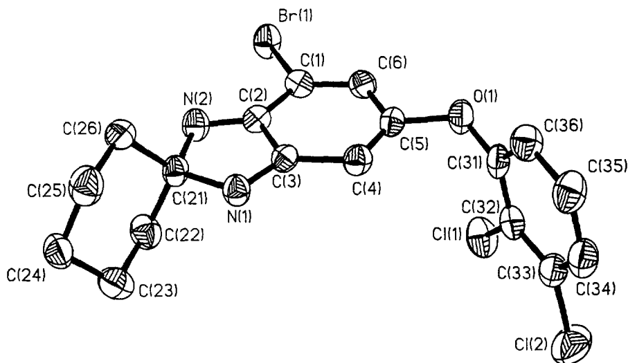
Fig. 1: Molecular structure of 4-bromo-6-(2,3-dichlorophenoxy)-2 H -benzimidazole-2-spirocyclohexane 2
